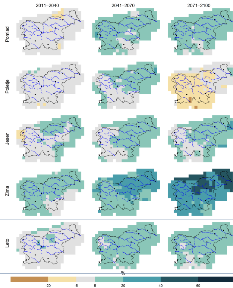
RCP8.5
